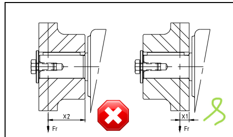
Drawing 6.2 Advise mounting.
