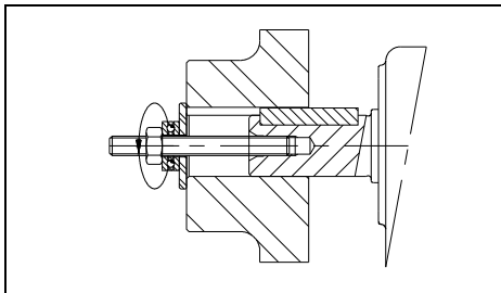
Drawing 6.1 Special tool.
